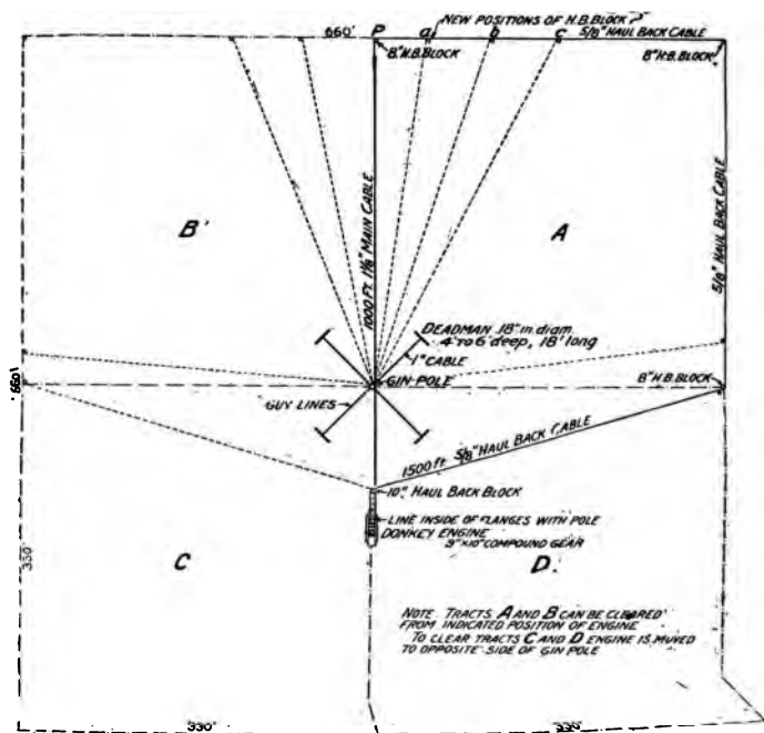
Fig. 52. Plan Showing Donkey Engine Rigged for Clearing L o
